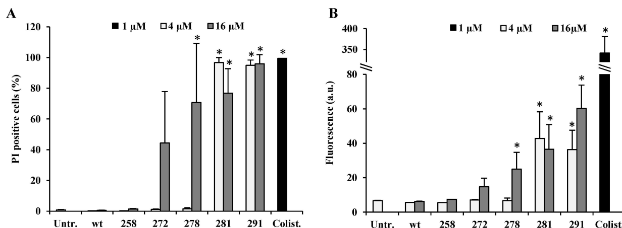
Figure 3. Flow cytometric evaluation of E. coli BW25113 membranes permeabilization. Propidium-iodide uptake assay was performed after 30 min incubation in the presence of 4 \mu M and 16 \mu M of peptides. (A) The percentage of permeabilized cell in the bacterial population and (B) the average fluorescence of permeabilized bacteria were assessed. 1 \mu M of the lytic antibiotic colistin (Colist.) was used as a positive control of permeabilization. In the untreated control (Untr.) bacteria were treated with sterile water. Average and standard deviation of three independent experiments. * = p-value < 0.05 versus the wt peptide (Student t-test).
