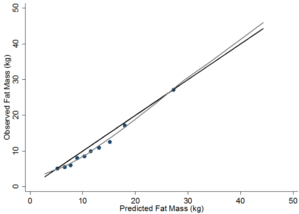
FIGURE 3: CALIBRATION PLOT OF MEAN OBSERVED AGAINST MEAN PREDICTED VALUES, ACROSS TENTHS OF PREDICTED FAT MASS, FROM EXTERNAL VALIDATION BEFORE RECALIBRATION OF INTERCEPT
